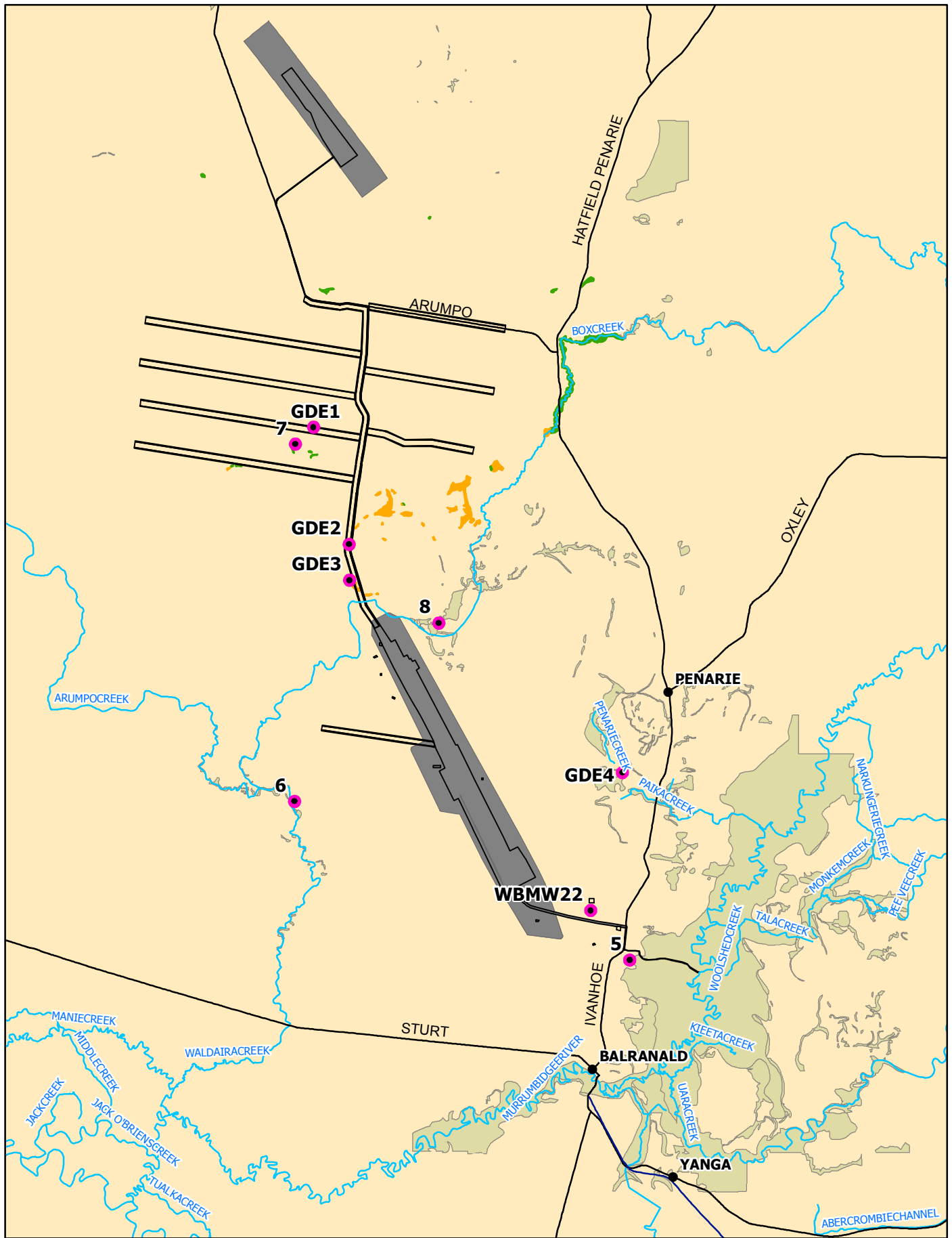
Figure 7-4: Mounding impact
