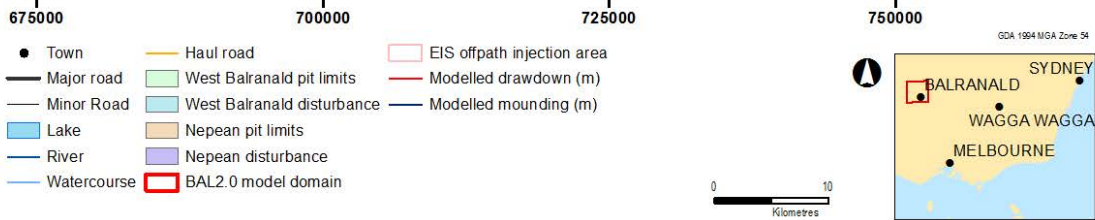
JACOBS BAL2.0 TS2 opt29 modelled drawdown in Shepparton Formation 30 years post-mining
