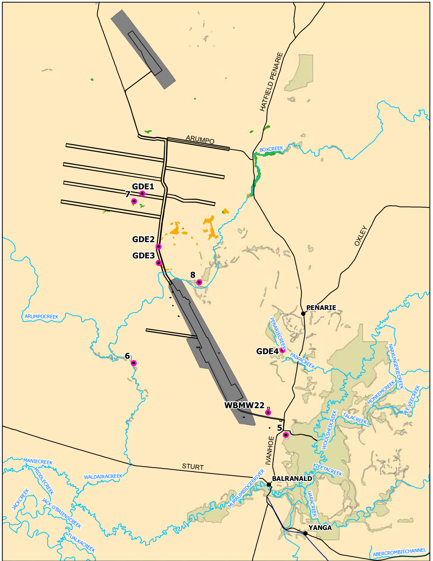
Figure 7-4: Mounding impact
