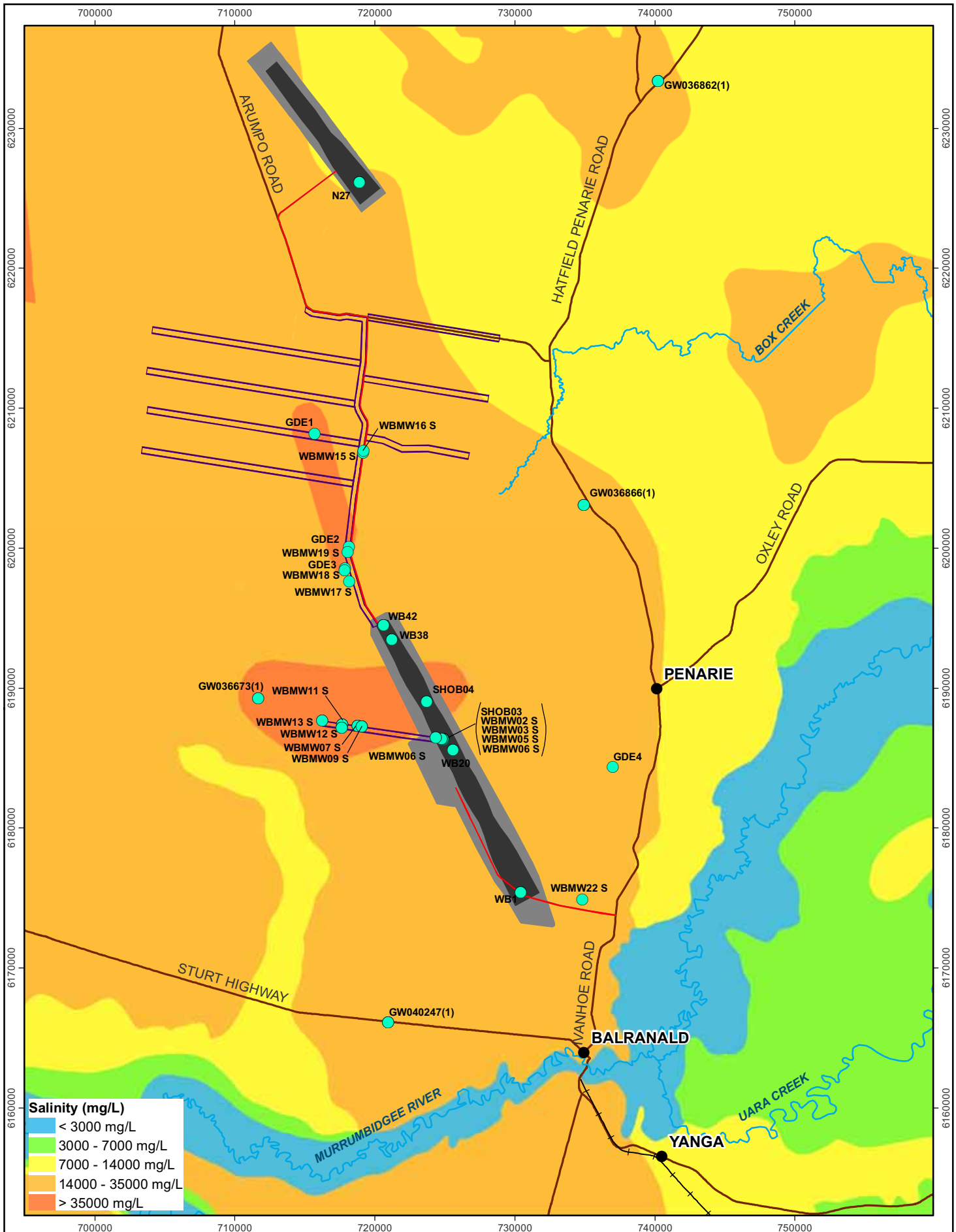
Figure 4-4: Salinity in the water table aquifer
