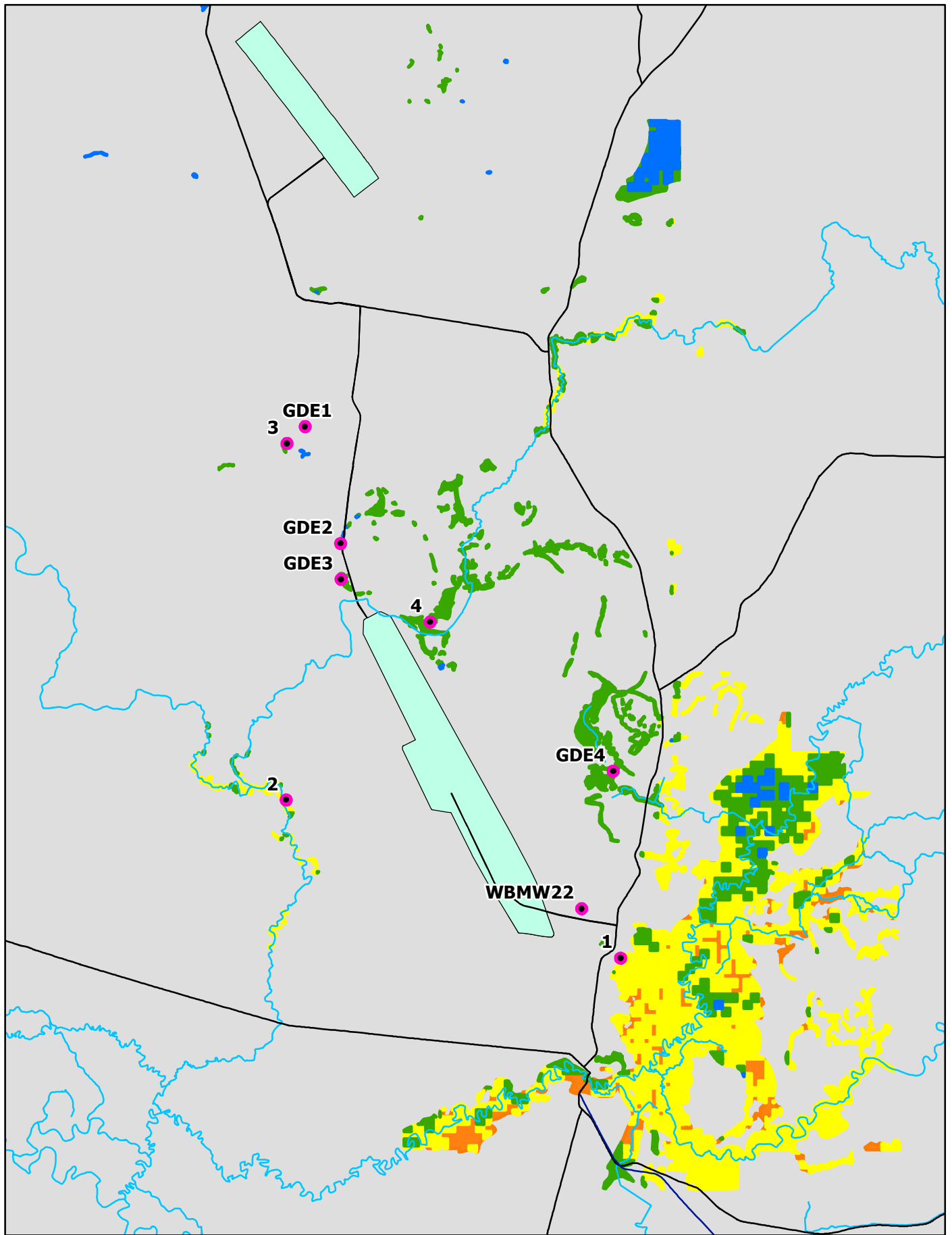
Figure 6-5: GDE Class
