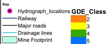
Figure 6-5: GDE Class
