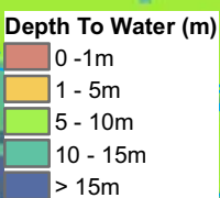
Figure 4-3: Modelled Baseline Depth To Water
