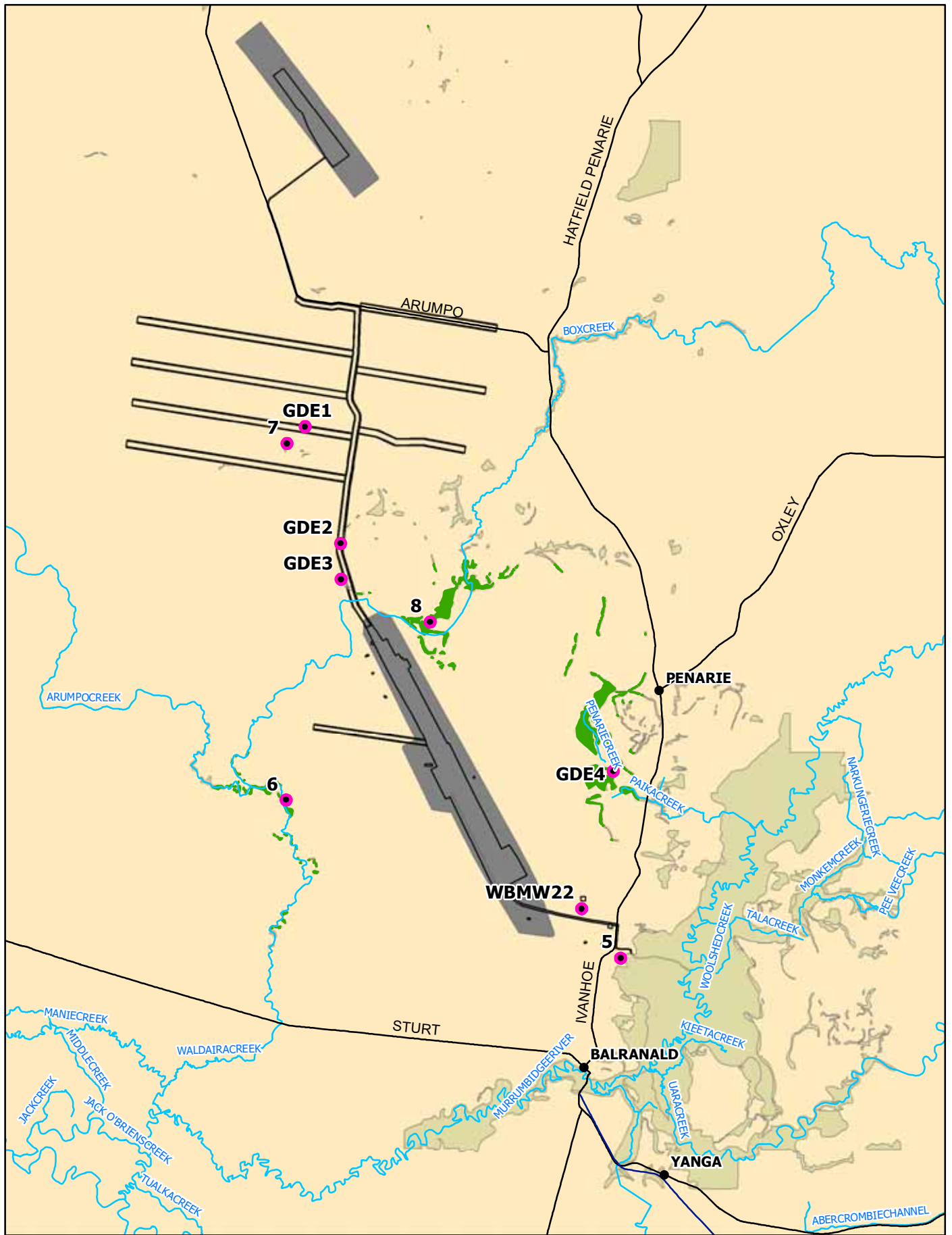
Figure 7-3: Drawdown impact
