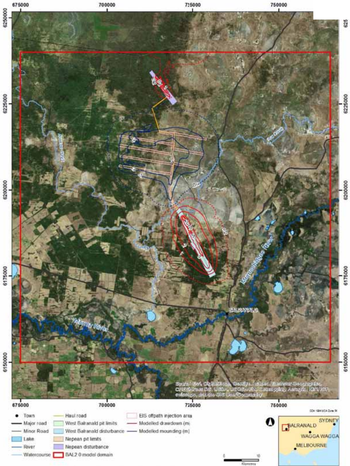
BAL2.0 TS2 opt29 modelled drawdown in Shepparton Formation at mining year 7.4 (maximum West Balranald dewatering rate)
