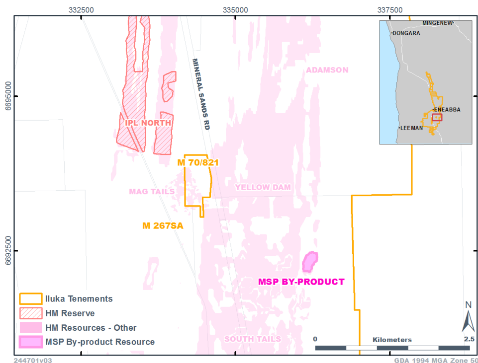
Figure 1: Eneabba summary plan showing the MSP By-Product Mineral Resource in relation to current infrastructure and HM Mineral Resources
