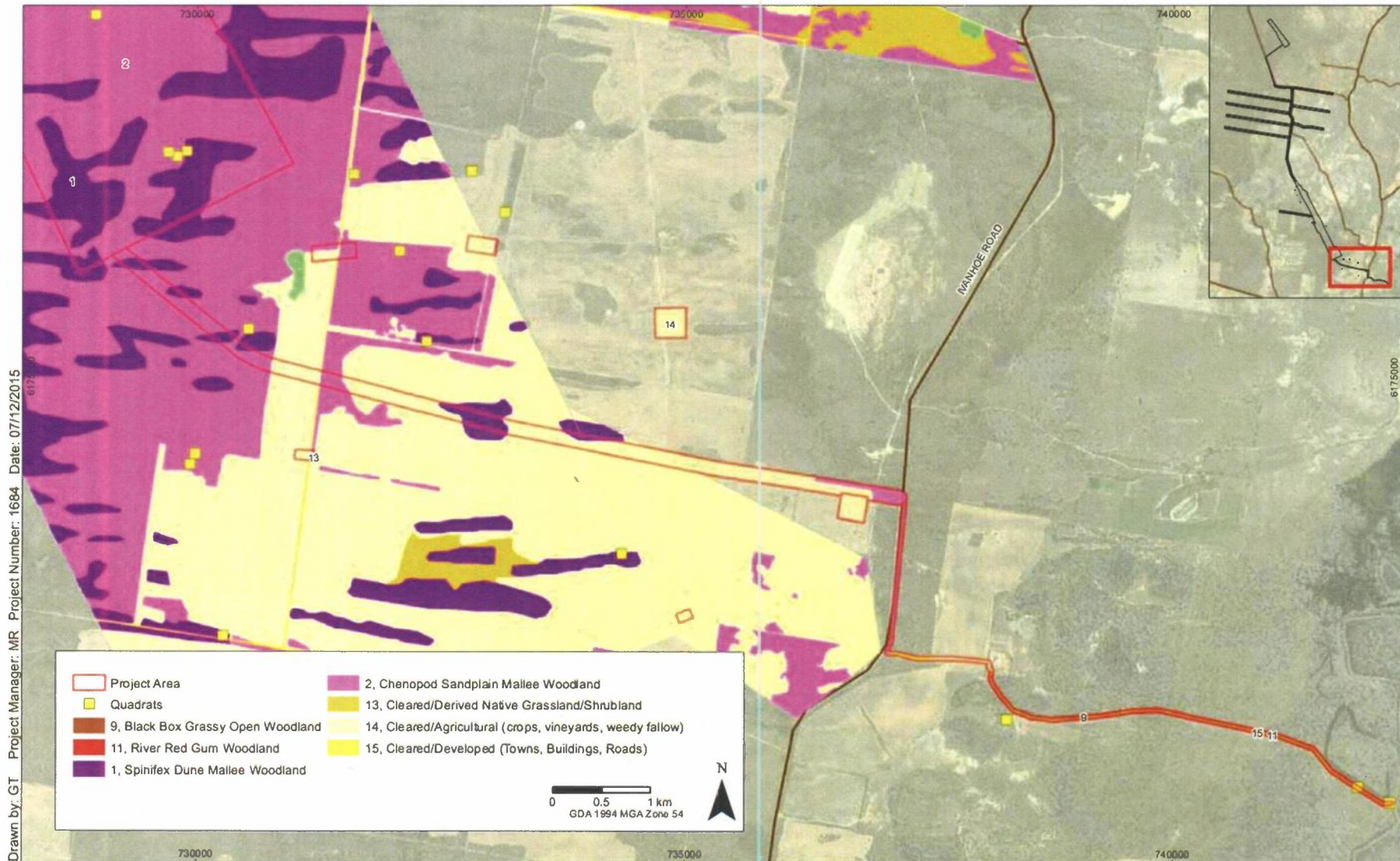
Vegetation community delination and Biometric plot locations for the Balranald Project (water supply pipeline area)
