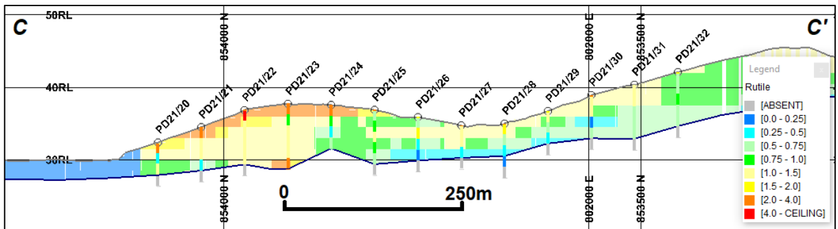
Figure 4: Pejebu drill hole and block model section showing in situ rutile grade (%) (looking east x10 VE).
