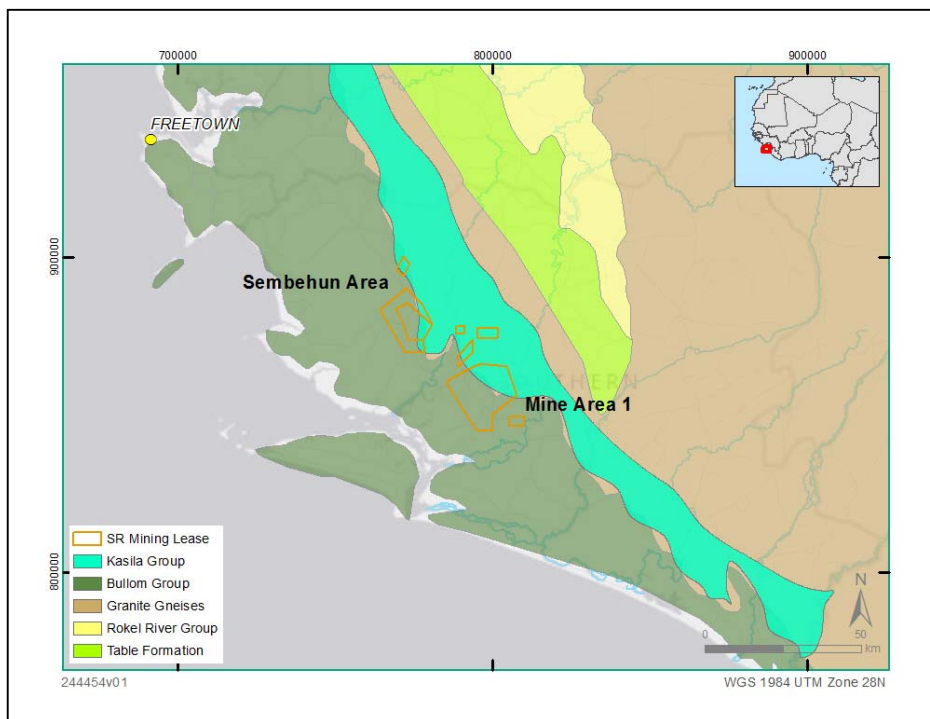
Figure 5: Regional Geology Plan for Sierra Leone.
