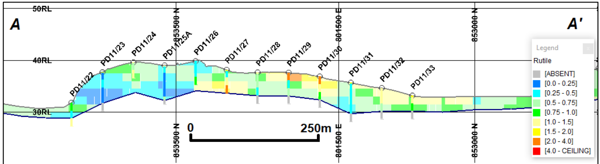
Figure 3: Pejebu drill hole and block model section showing in situ rutile grade (%) (looking east x10 VE).
