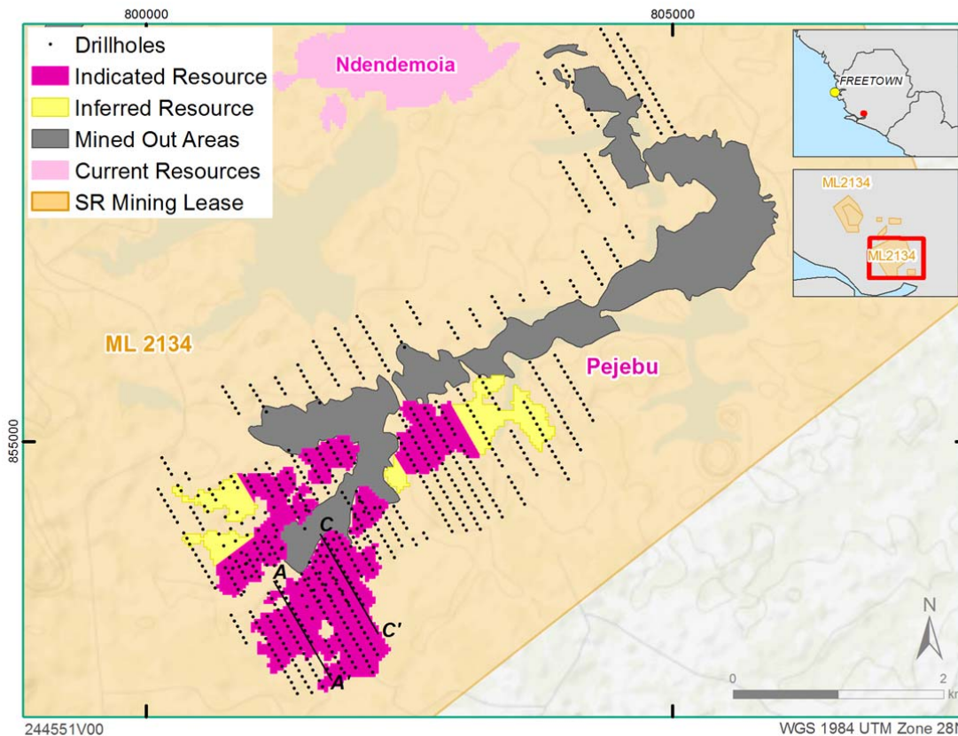
Figure 2: Pejebu drill collar locations and JORC Category distribution. The locations for cross section A – A' (Figure 3) and C – C' (Figure 4) are shown.
