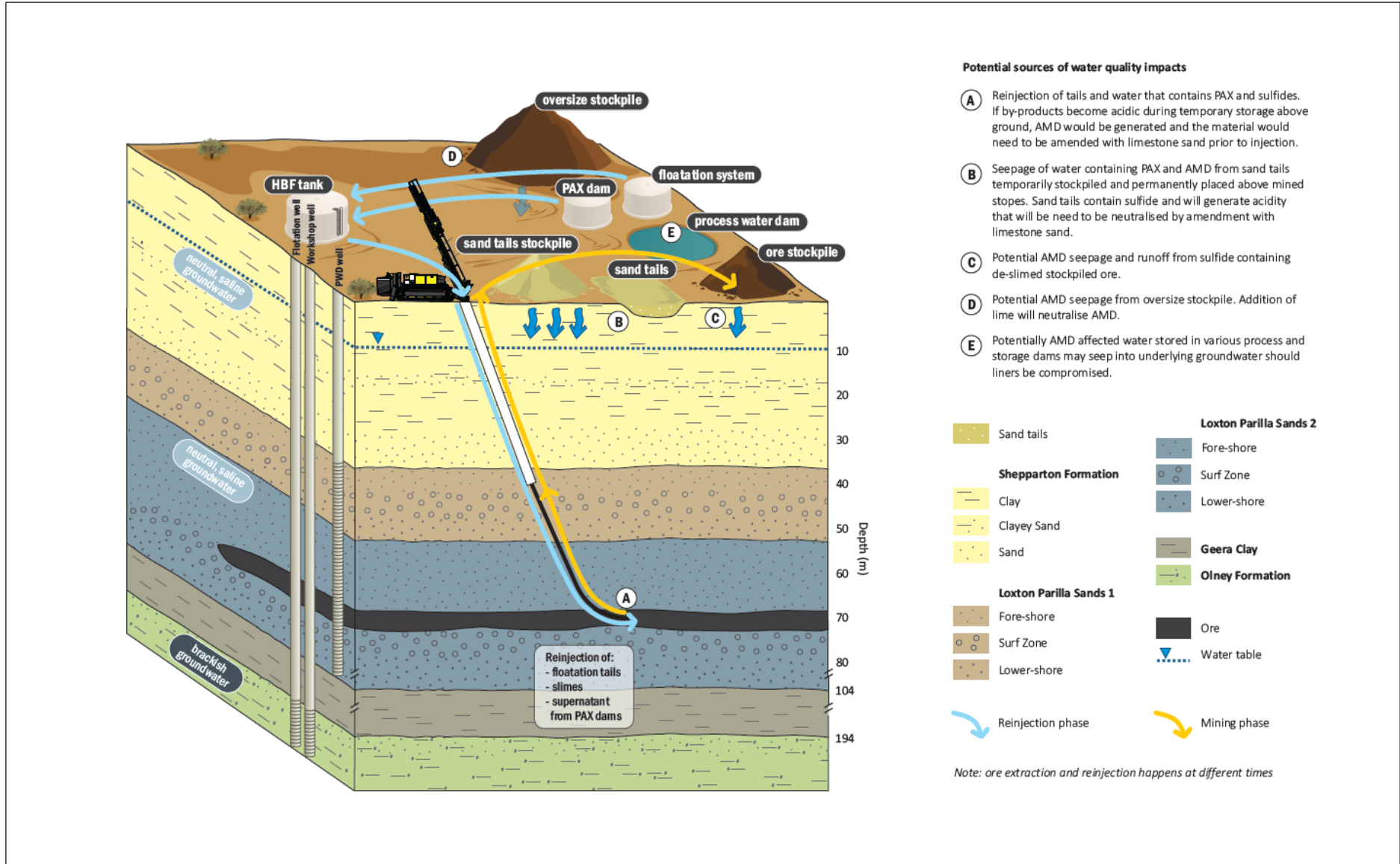
Figure 5- Mining process
