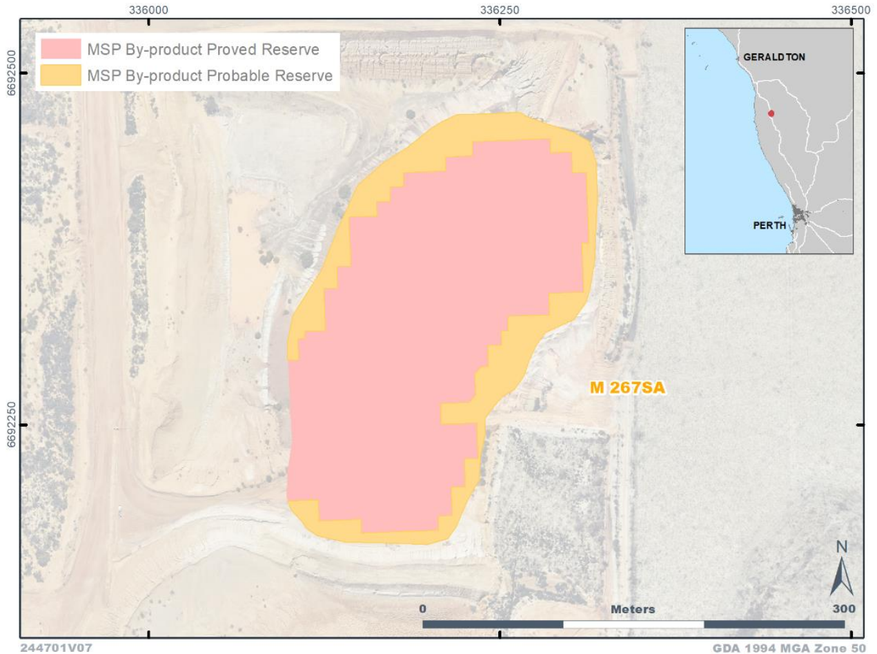
Figure 2: MSP By-Product Ore Reserve JORC category distribution.
