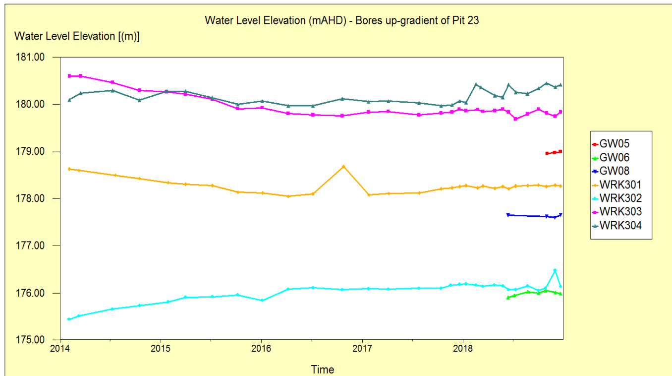
Figure 21: Groundwater elevation (mAHD) – bores up-gradient of Pit 23
