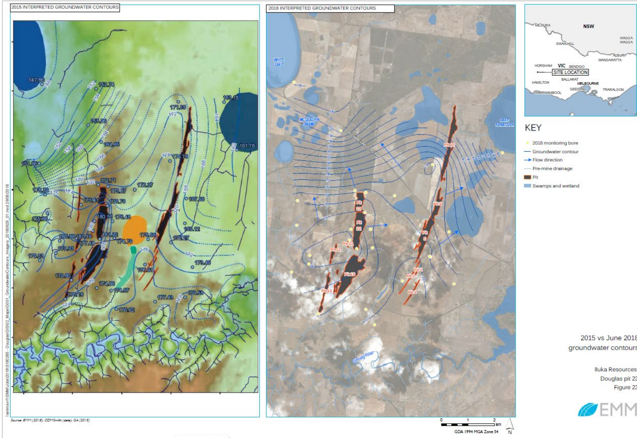
Figure 23: Douglas Groundwater contours and flow paths, 2015 Modelled vs 2018
