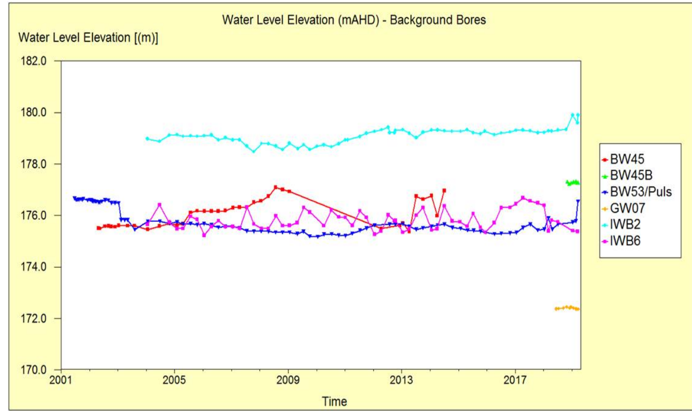
Figure 22: Groundwater elevation (mAHD) – cross-gradient and background bores
