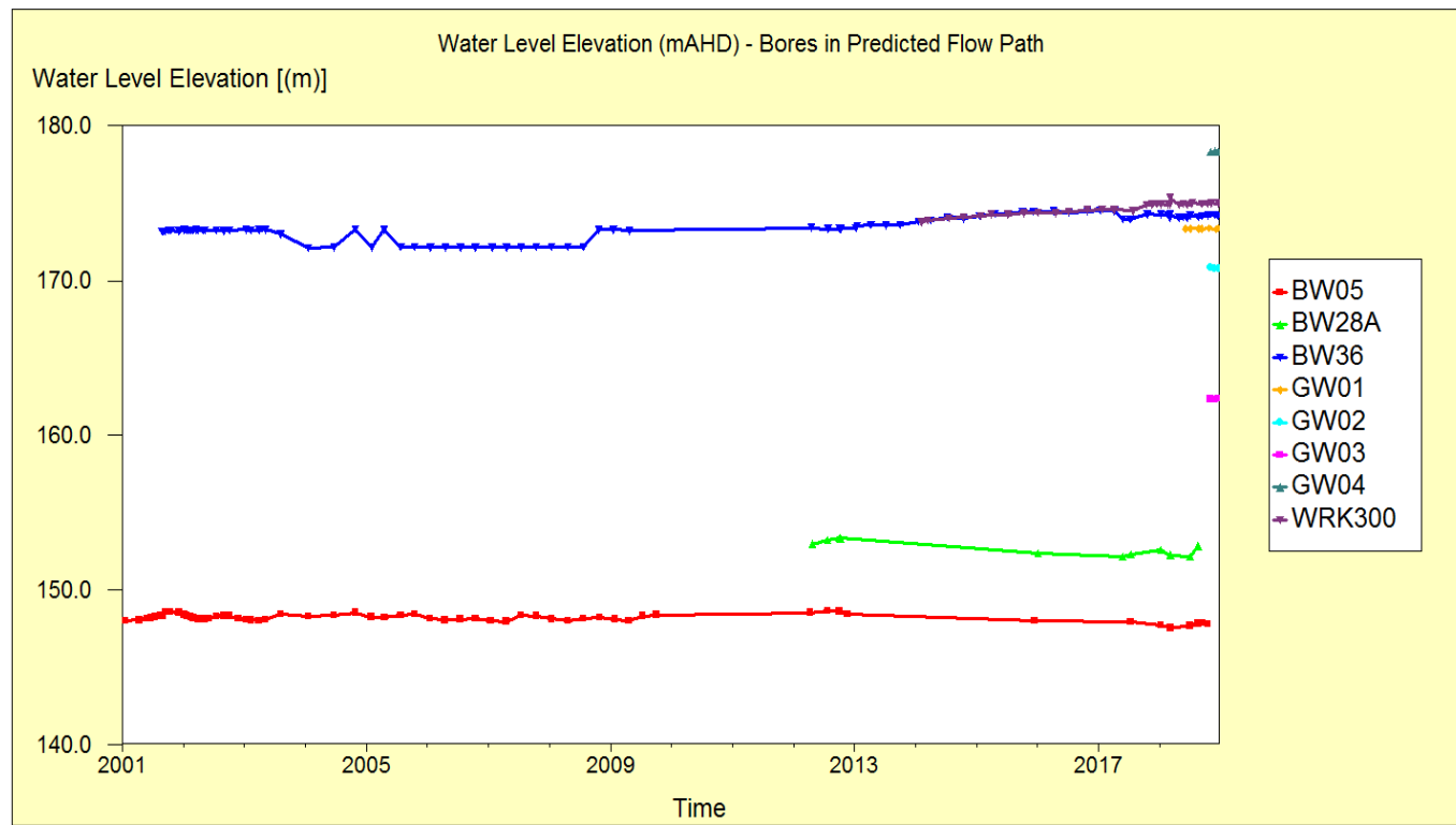
Figure 20: Groundwater elevation (mAHD) – bores in predicted flow path
