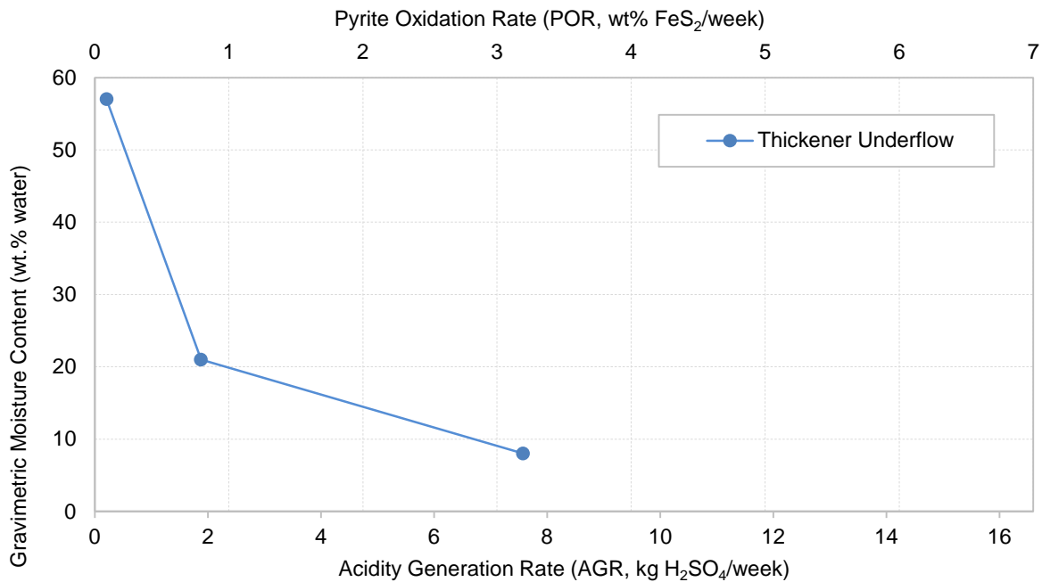
Figure 28: Pyrite oxidation rate (POR) and acidity generation rates (AGR) vs. gravimetric moisture content (GMC) for Balranald thickener underflow samples, showing inferred trend (Earth Systems, 2015).
