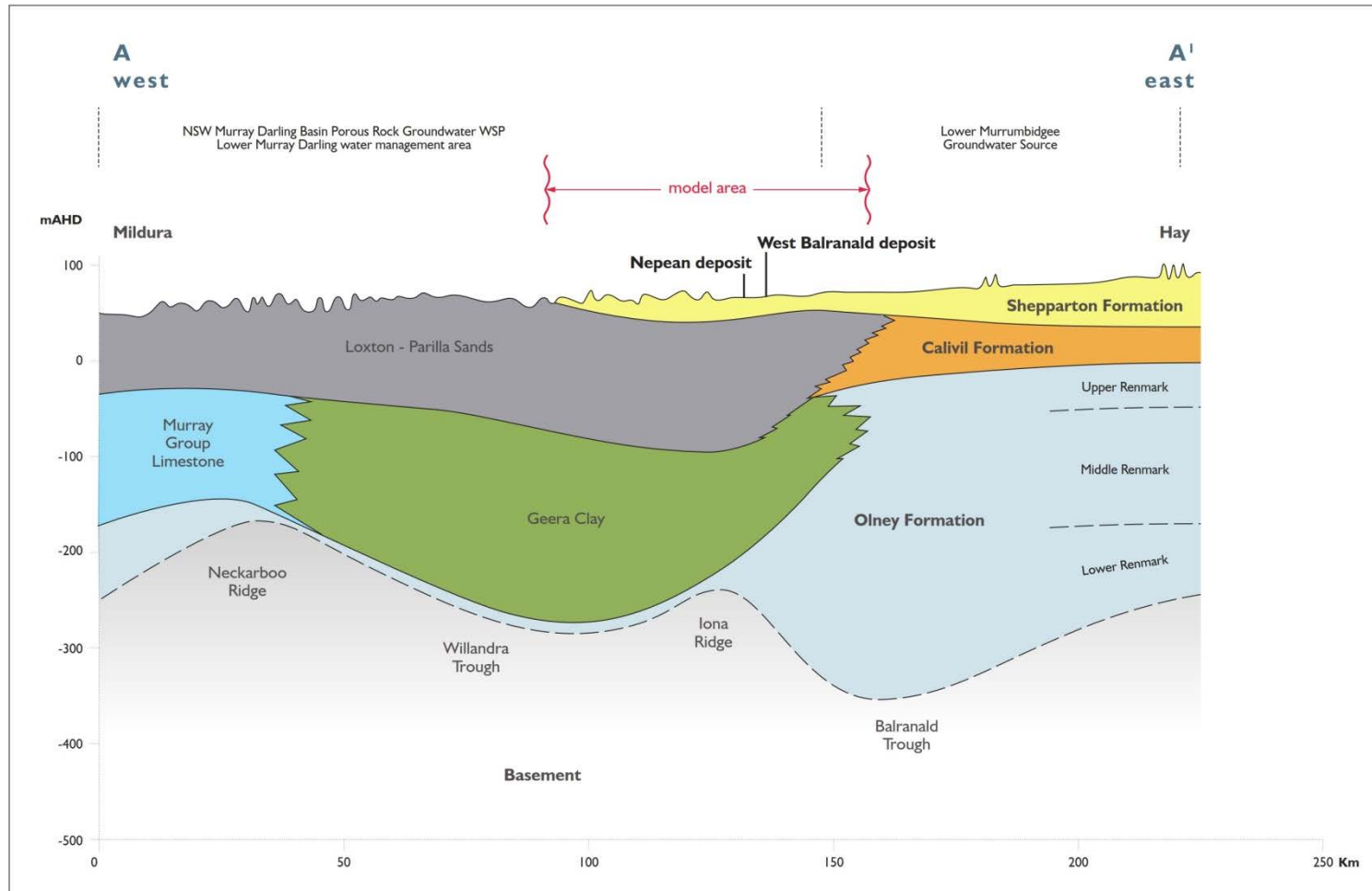
Conceptual geology of the Murray Basin Balranald Miner Sands Project Water Assessment
