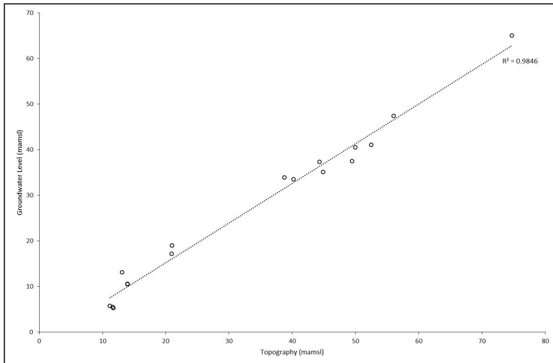
Figure 8-3: SR Area 1 Topography vs Groundwater Level (mamsl)
