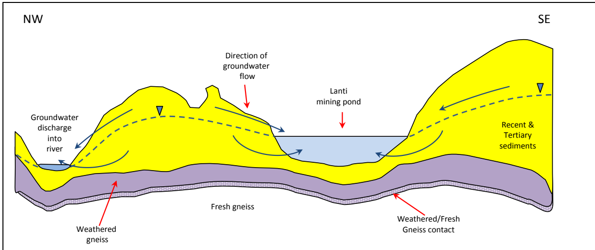
Figure 10-3: Lanti Mining Pond Groundwater Flow Patterns
