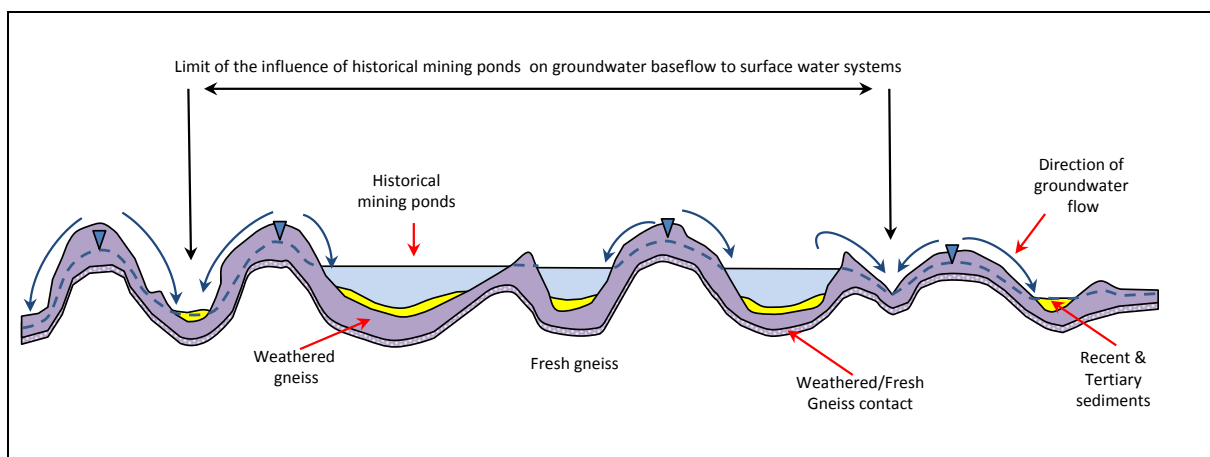
Figure 10-2: Historical Mining Pond Groundwater Flow Patterns
