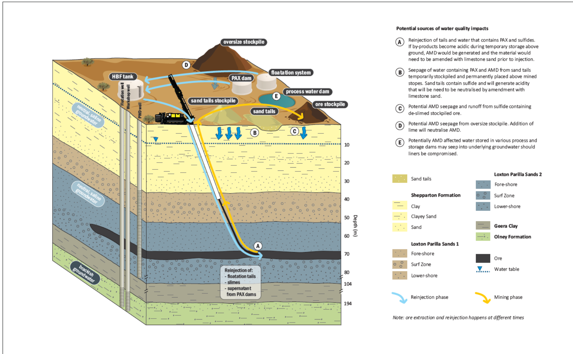
Figure 5- Underground mining process
