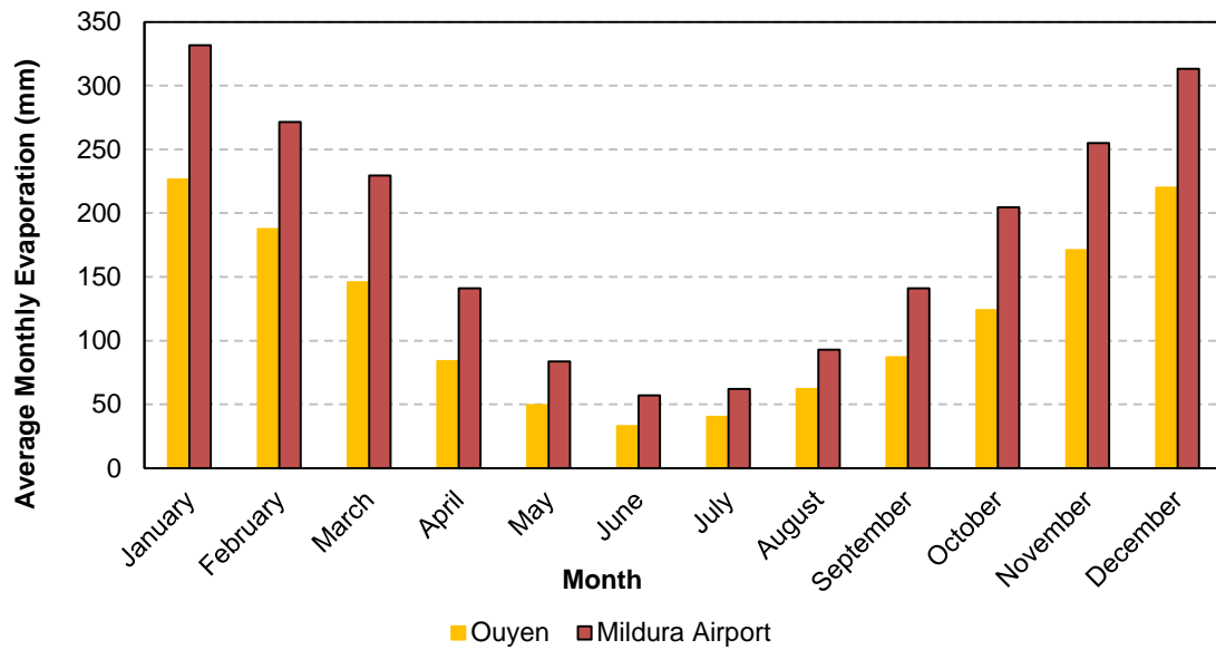
Figure 9: Average monthly pan evaporation (mm/month) at Ouyen (1972-1987) and Mildura Airport (1965-2014; BOM, 2014).
